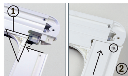
Installation around existing hatch trim.
